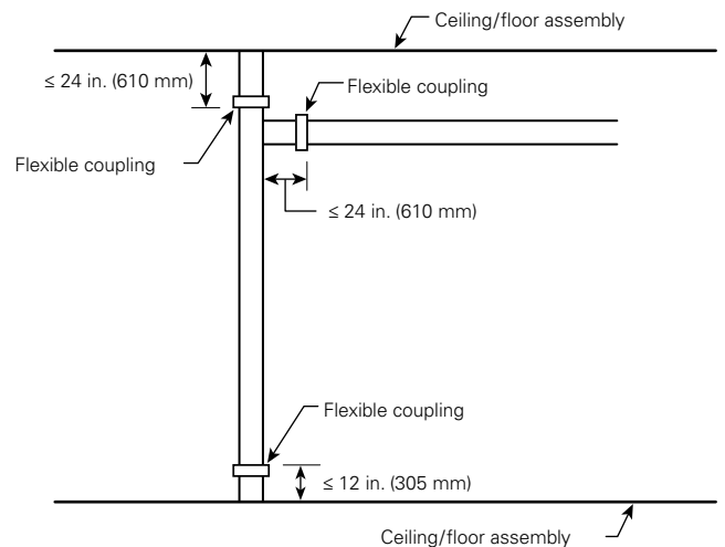
FIGURE A.9.3.2(2) Flexible Coupling on Horizontal Portion of Tie-In.
